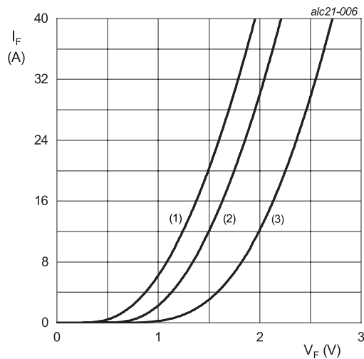
(1) T J = 150 °C; typical values (2) T J = 150 °C; maximum values (3) T J = 25 °C; maximum values V 0 = 0.943 V; R s = 0.0273 Ω
