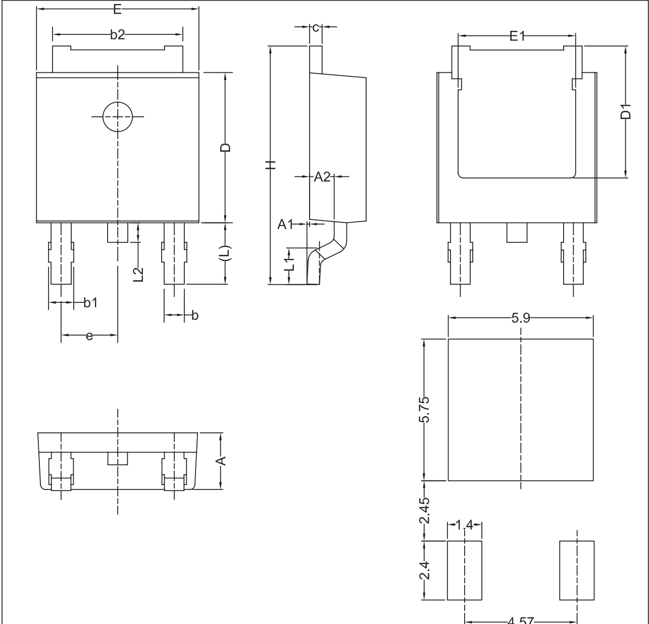
Recommended Footprint
