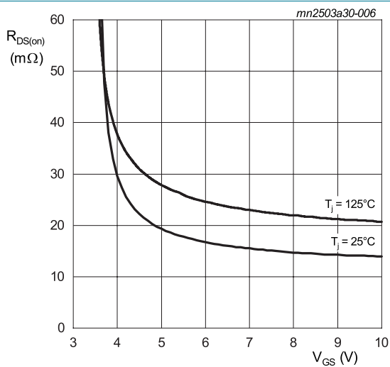
I_D = 14 A Fig. 6. Drain-source on-state resistance as a function of gate-source voltage; typical values
