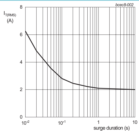
f = 50\text{ Hz} ; T_{sp} = 117\text{ °C} Fig. 2. RMS on-state current as a function of surge duration; maximum values
