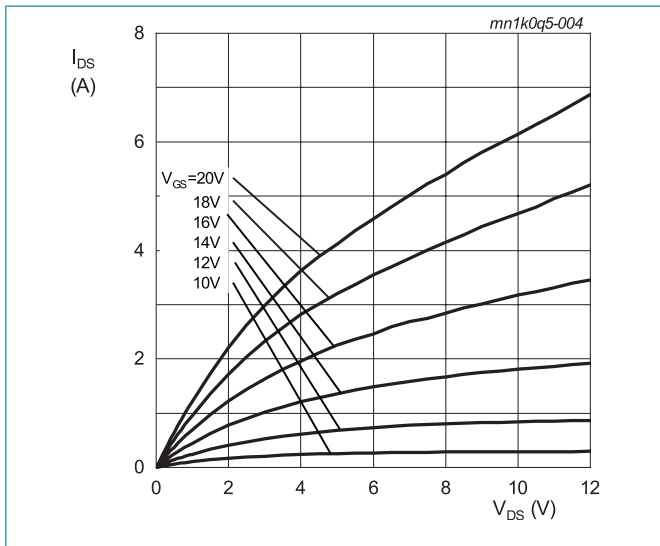
T_j = -55\text{ °C}; t_p < 200\ \mu\text{s} Fig. 4. Output characteristics; drain current as a function of drain-source voltage; typical values
