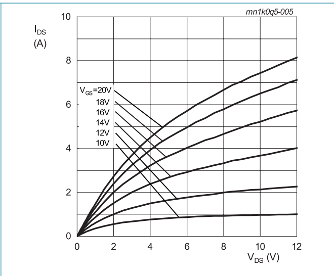
T_j = 25\text{ °C}; t_p < 200\ \mu\text{s} Fig. 5. Output characteristics; drain current as a function of drain-source voltage; typical values
