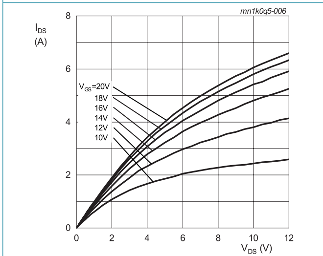
T_j = 150\text{ °C}; t_p < 200\ \mu\text{s} Fig. 6. Output characteristics; drain current as a function of drain-source voltage; typical values
