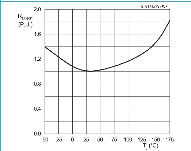
I_{DS} = 1\text{ A}; V_{GS} = 18\text{ V}; t_p < 200\ \mu\text{s} Fig. 7. Normalized drain-source on-state resistance as a function of junction temperature
