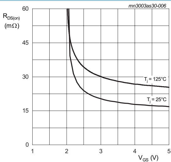
I_D = 14\text{ A} Fig. 6. Drain-source on-state resistance as a function of gate-source voltage; typical values
