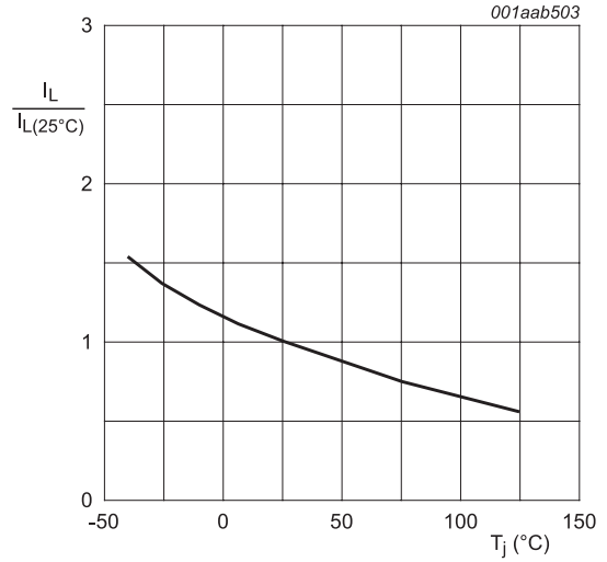
Fig. 8. Normalized latching current as a function of junction temperature R_{GK} = 1 \text{ k}\Omega
