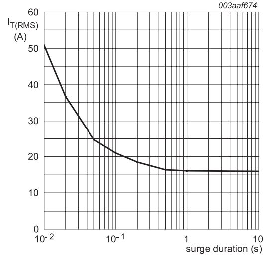
f = 50 Hz; T_{mb} = 126^{\circ}C Fig. 3. RMS on-state current as a function of surge duration; maximum values
